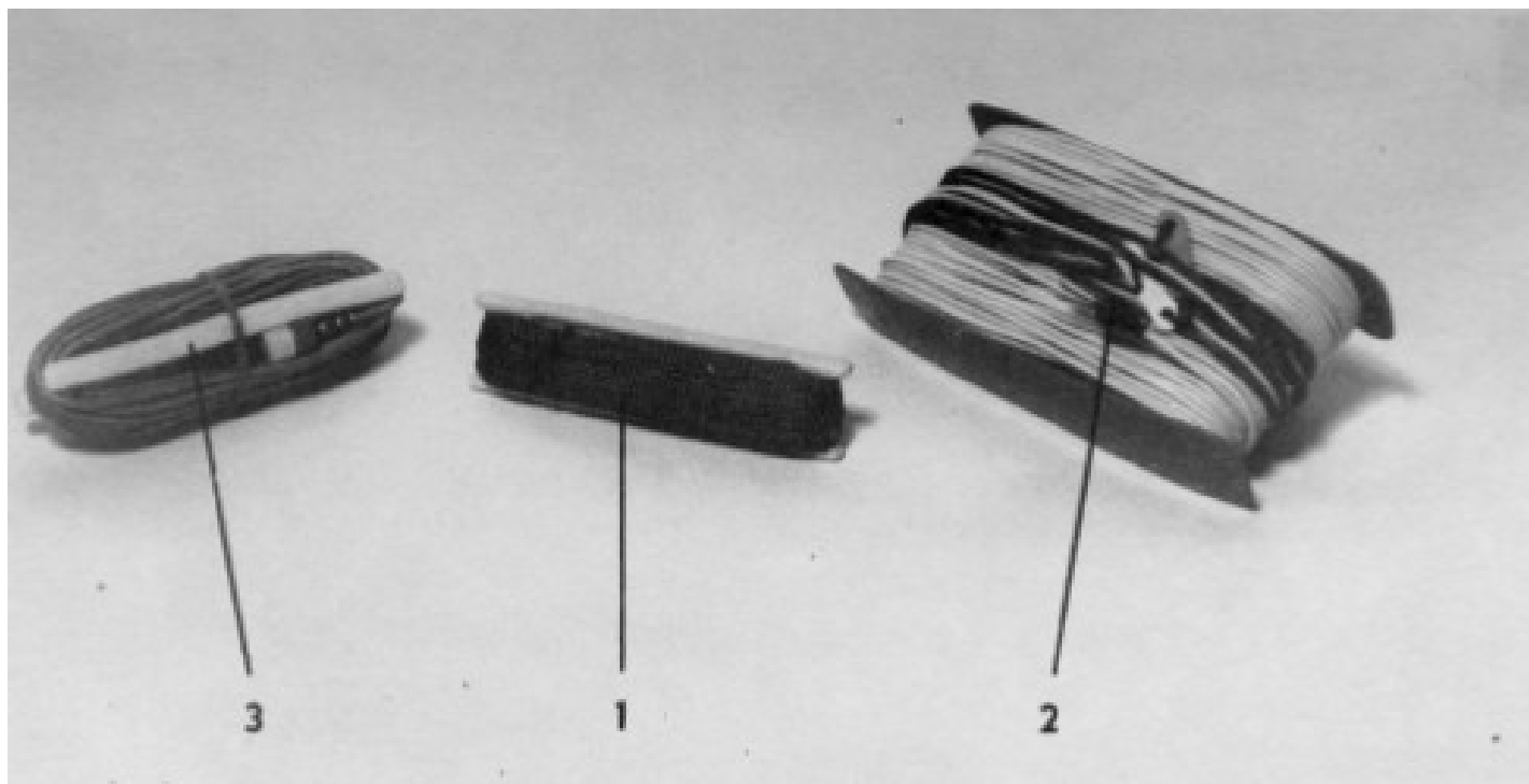
Figure 15: Wire antennas 1 – suspension cord; 2 – directional antenna; 3 – suspension antenna
