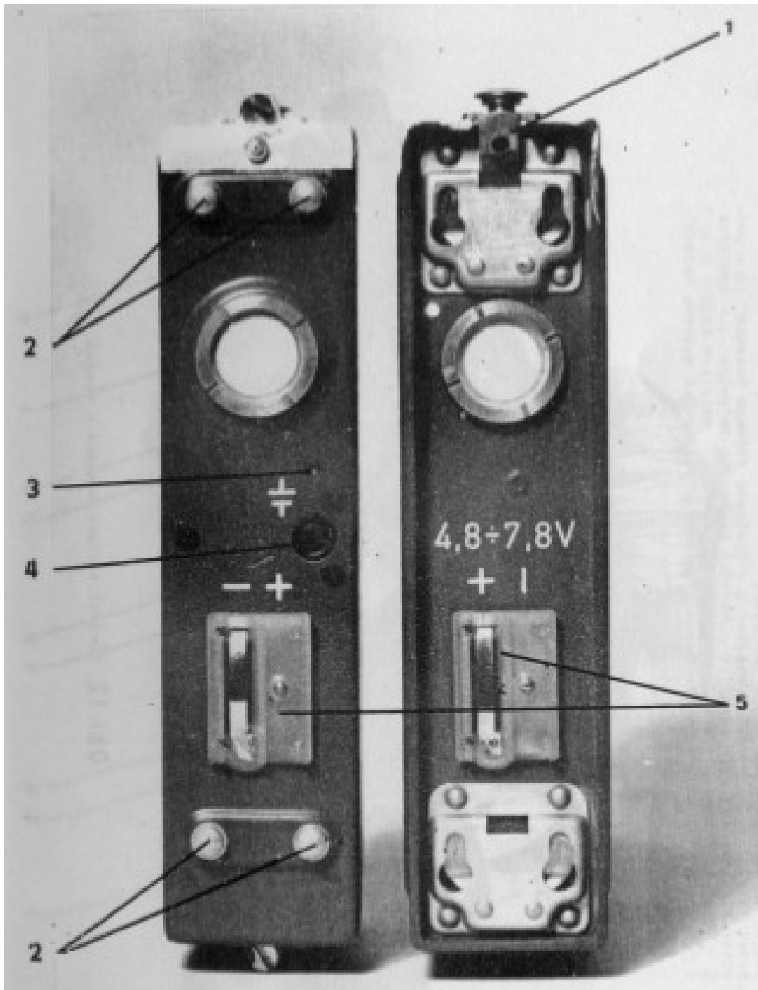
Figure 11: Battery pack lid and bottom of radio set 1 – locking spring; 2 – spigot pins; 3 – indicator light; 4 – test button; 5 – battery connector (Battery packs QN 732 10 produced after September 1, 1979 do not have items 3 & 4
