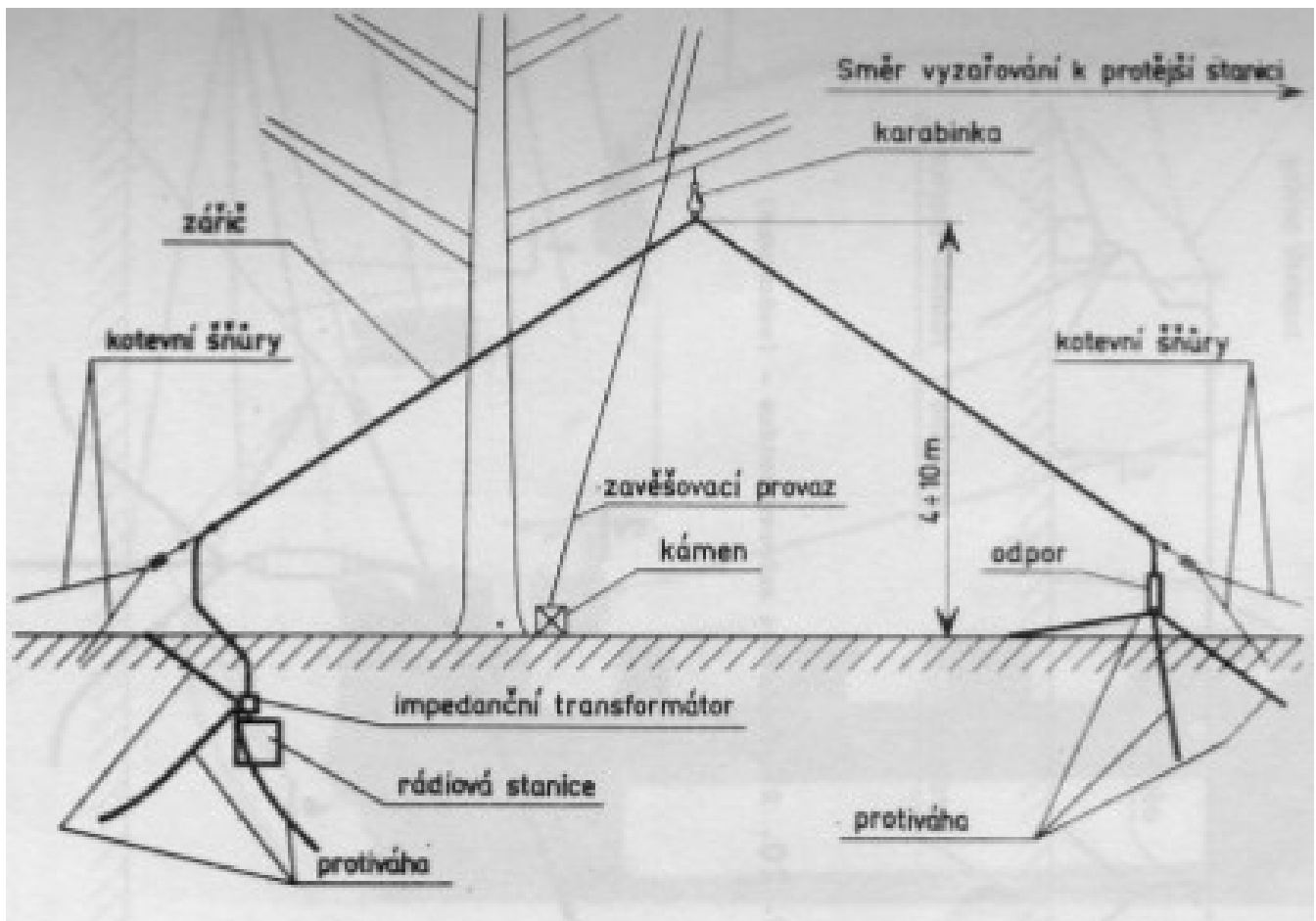
Figure 19: Directional antenna – half-rhombic
