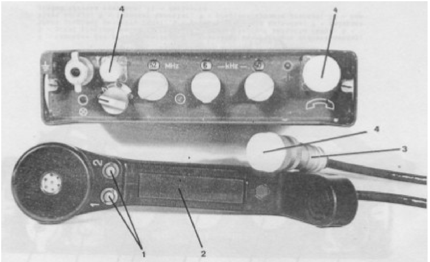
Figure 14: Radio set and handset 1 – push buttons; 2 – PTT switch; 3 – 19-pin connector; 4 – protective caps
