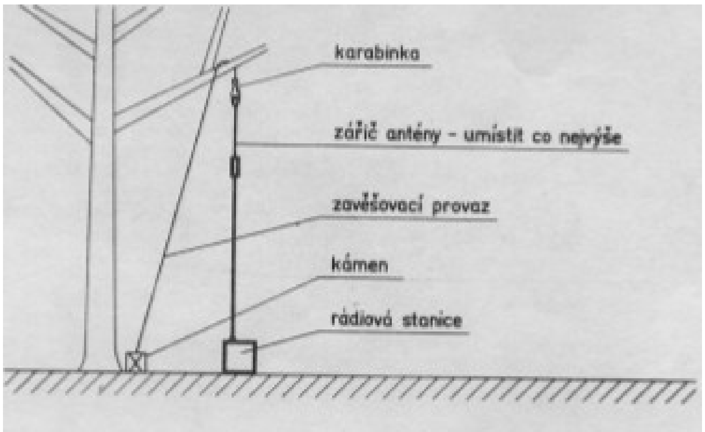
Figure 18: Suspension antenna
