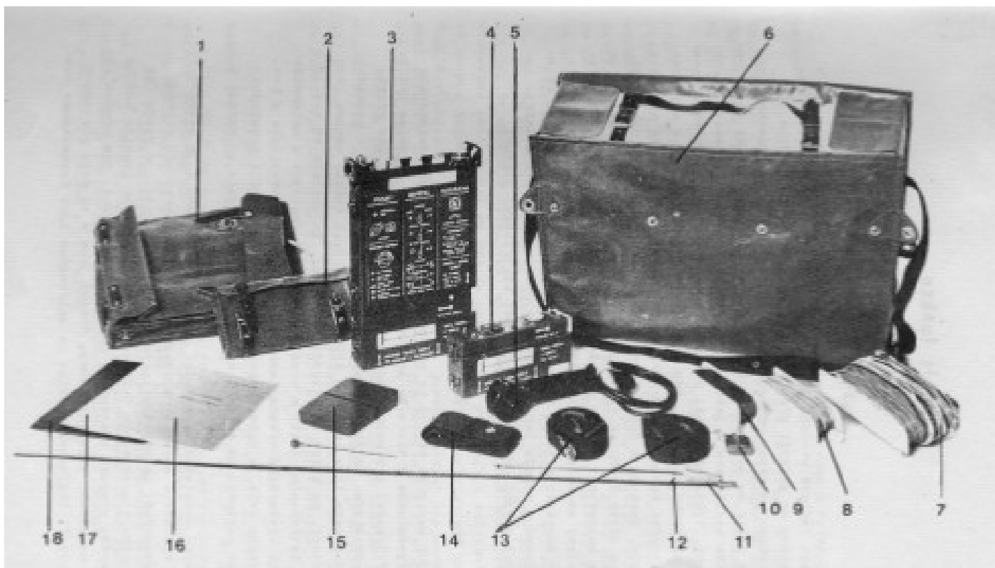
Figure 1: Complete radio set kit
