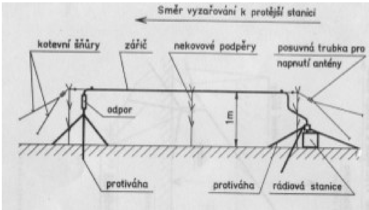
Figure 20: Horizontal directional antenna – (horizontal)
