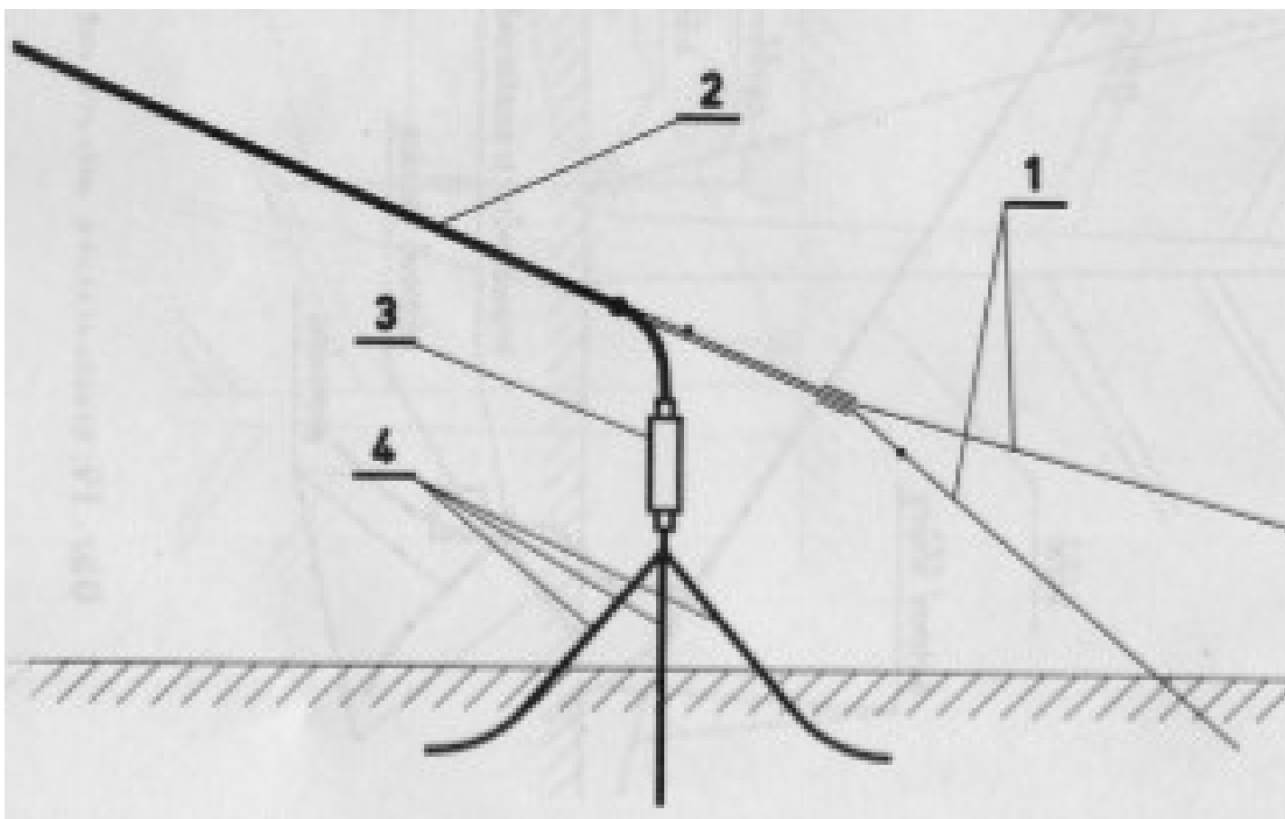
Figure 21: Terminating resistor with radials 1 – guy ropes; 2 – part of the radiator; 3 – terminating resistor; 4 – radials
